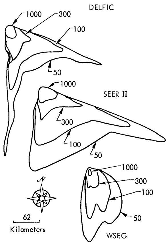
Fig. 8. Comparison of fallout patterns for a 1-Mt detonation. (From Ref. 14.)
